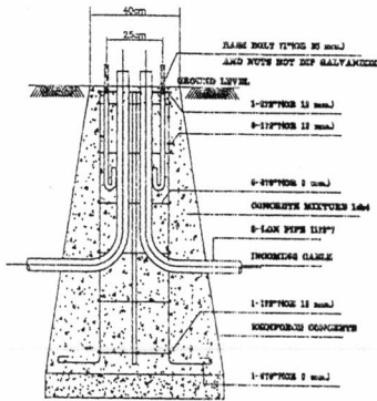
TYPICAL CONCRETE FOUNDATION & BASE BOLT
