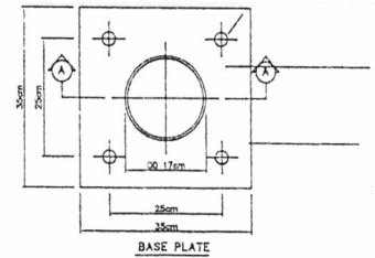
BASE PLATE
